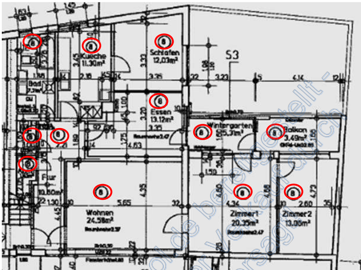
Grundriss WE 8
