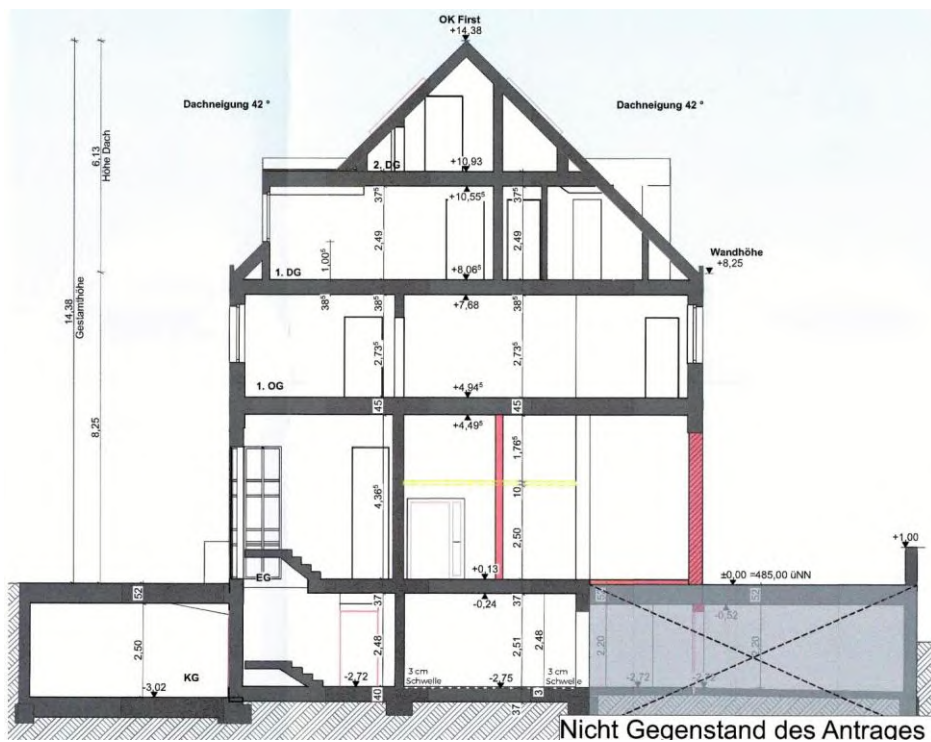
Schnitt Ost-West
