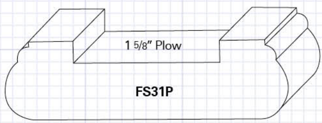
FS31P Poplar Shoe Rail / Pine FJ 7/8" x 3 1/8" (1 5/8" Plow)
