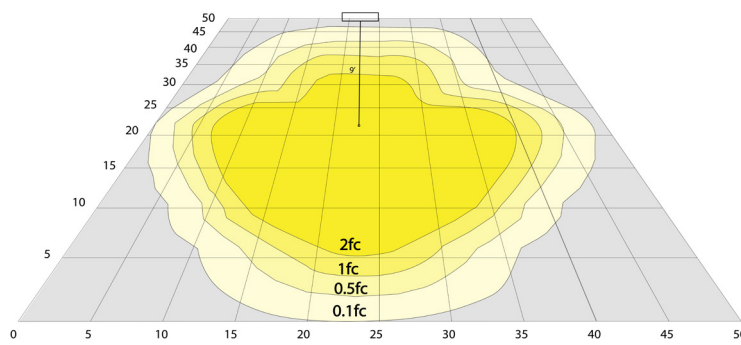
Area 45'x 50' Mounting Height: 9'
