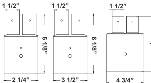
DAB-PA2-2 2 1/4"(W) x 6 1/8"(H) DAB-PA3-2 3 1/2"(W) x 6 1/8"(H) DAB-PA4-2 4 3/4"(W) x 7"(H)
