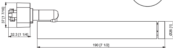
Technical Drawing: 1" (D) × 7-1/2" (H) Overall fixture height: 7-1/2"
