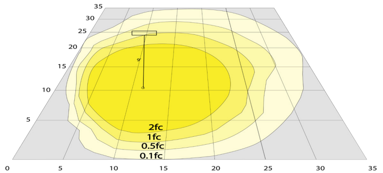
10W, 5000K Area 35'x 35' Mounting Height: 9'
