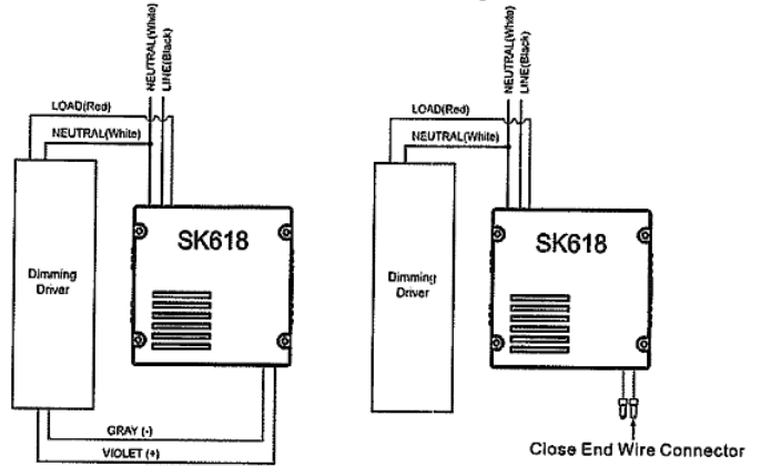
SK618 wiring with Dimming ballast or LED driver.
