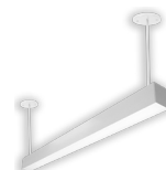
Suspension Rod Kit SCL-RS-12 12" SCL-RS-18 18" SCL-RS-24 24" SCL-RS-36 36" SCL-RS-48 48"
