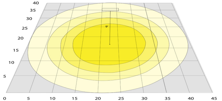
Area 40' x 45' Mounting Height: 9'
