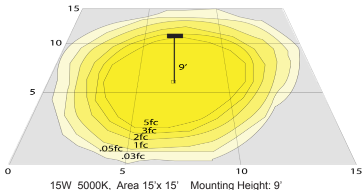
15W 5000K, Area 15'x 15' Mounting Height: 9'
