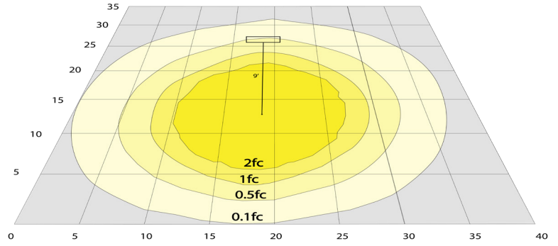
Area 30'x 40' Mounting Height: 9'
