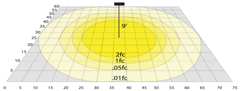
80W 5000K, Area 60'x 75' Mounting Height: 9'
