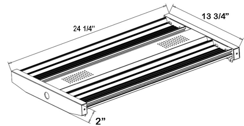
24 1/4" (L) X 13 3/4" (W) X 2" (H)
