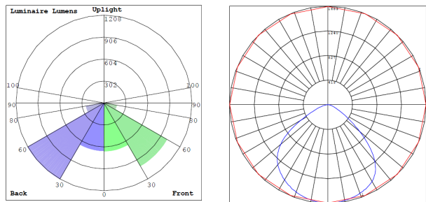
BUG Rating: B2-U0-G1
