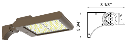
LFX-ASA Adjustable Straight Arm 3 1/3" x 7 7/8"
