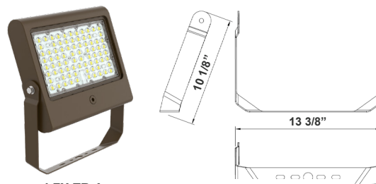
LFX-TR-A U Bracket 13 3/8" x 10 1/8"
