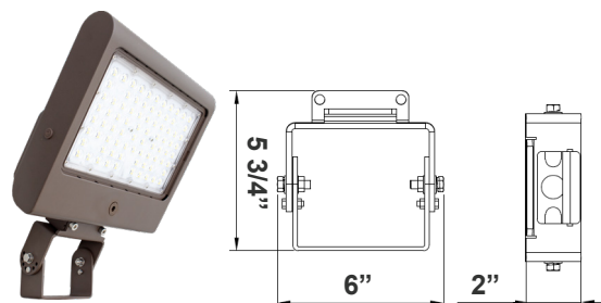
LFX-YK Yoke 5 3/4" x 6" x 2"
