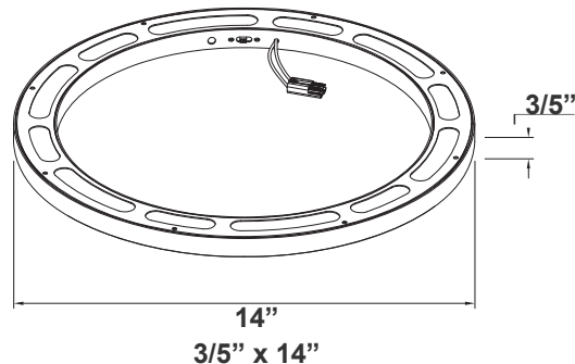
FML-ULK-MCT 15W, 850LM, 30K/40K/50K UP LIGHT KIT
