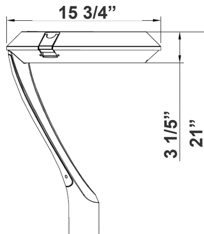
15 3/4" (W) X 21"(H) Inside Diameter: 2 3/4"
