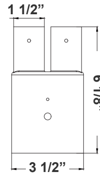
DAB-PA3-2 3 1/2"(W) x 6 1/8"(H)
