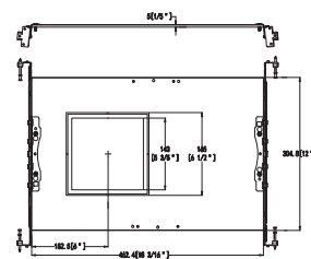
CRLCS-46-RIBH-JB CRLC Square Mounting Plate With Brackets And J-Box 4/6 in
