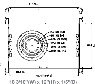
CRLC-468-RIBH-JB CRLC Series Mounting Plate With Brackets And J-Box 4/6/8 in
