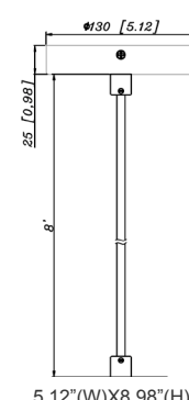
5.12" (W) X 8.98" (H) 11.81" (W) X 5.59" (H) X 13.46" (H) CMC4-MCTP-DD-BK+CMC-CS-8FT-BK+CMC4-FS14-BG CMC4-MCTP-DD-WH+CMC-CS-8FT-WH+CMC4-FS14-WG
