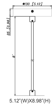
5.12" (W) X 8.98" (H) 6.7" (W) X 4.59" (D) CMC4-MCTP-DD-BK+CMC-CS-8FT-BK+CMC4-WPCK-BK CMC4-MCTP-DD-WH+CMC-CS-8FT-WH+CMC4-WPCK-WH
