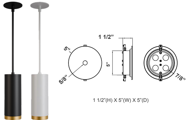
CMC4-MCTP-DD-BK+CMC-OWCC-BK+CMC-SRK-218-5C-BK CMC4-MCTP-DD-WH+CMC-OWCC-WH+CMC-SRK-218-5C-WH
