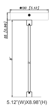
CMC4-MCTP-DD-BK+CMC-CS-8FT-BK+CMC4-WPCK-BK CMC4-MCTP-DD-WH+CMC-CS-8FT-WH+CMC4-WPCK-WH
