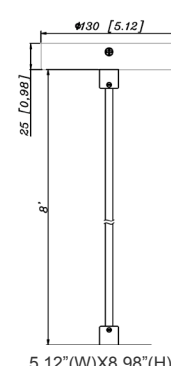
CMC4-MCTP-DD-BK+CMC-CS-8FT-BK+CMC4-FS14-BG CMC4-MCTP-DD-WH+CMC-CS-8FT-WH+CMC4-FS14-WG
