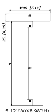
CMC4-MCTP-DD-BK+CMC-CS-8FT-BK+CMC4-FS14-BG CMC4-MCTP-DD-WH+CMC-CS-8FT-WH+CMC4-FS14-WG
