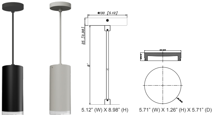
CMC4-MCTP-DD-BK+CMC-CS-8FT-BK+CMC4-DL32 CMC4-MCTP-DD-WH+CMC-CS-8FT-WH+CMC4-DL32
