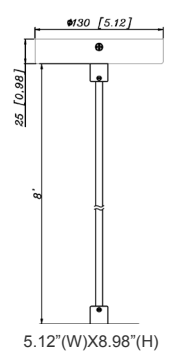
CMC4-MCTP-DD-BK+CMC-CS-8FT-BK+CMC4-WPCK-BK CMC4-MCTP-DD-WH+CMC-CS-8FT-WH+CMC4-WPCK-WH
