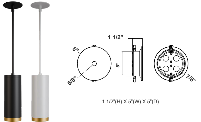
CMC4-MCTP-DD-BK+CMC-OWCC-BK+CMC-SRK-218-5C-BK CMC4-MCTP-DD-WH+CMC-OWCC-WH+CMC-SRK-218-5C-WH
