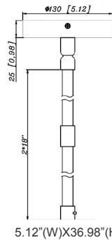
CMC4-MCTP-DD-BK+CMC-SRK-218-5C-BK CMC4-MCTP-DD-WH+CMC-SRK-218-5C-WH
