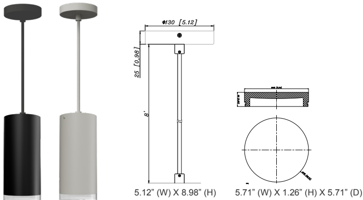
CMC4-MCTP-DD-BK+CMC-CS-8FT-BK+CMC4-DL32 CMC4-MCTP-DD-WH+CMC-CS-8FT-WH+CMC4-DL32
