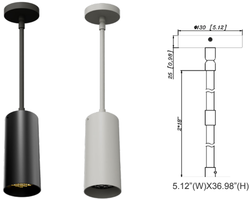
CMC4-MCTP-DD-BK+CMC-SRK-218-5C-BK+CMC4-HCDK-AG CMC4-MCTP-DD-WH+CMC-SRK-218-5C-WH+CMC4-HCDK-BK
