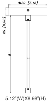
CMC4-MCTP-DD-BK+CMC-CS-8FT-BK+CMC4-DS14-BG CMC4-MCTP-DD-WH+CMC-CS-8FT-WH+CMC4-DS14-WG
