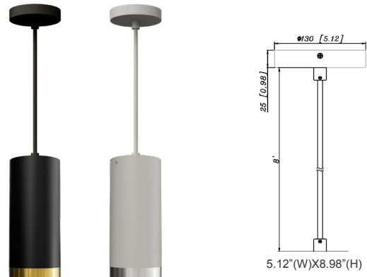
CMC4-MCTP-DD-BK+CMC-CS-8FT-BK+CMC4-TRM-AG CMC4-MCTP-DD-WH+CMC-CS-8FT-WH+CMC4-TRM-BN
