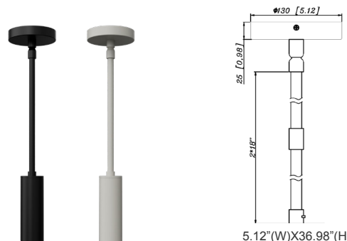
CMC2-MCT-DT-BK+CMC-SRK-218-5C-BK CMC2-MCT-DT-WH+CMC-SRK-218-5C-WH
