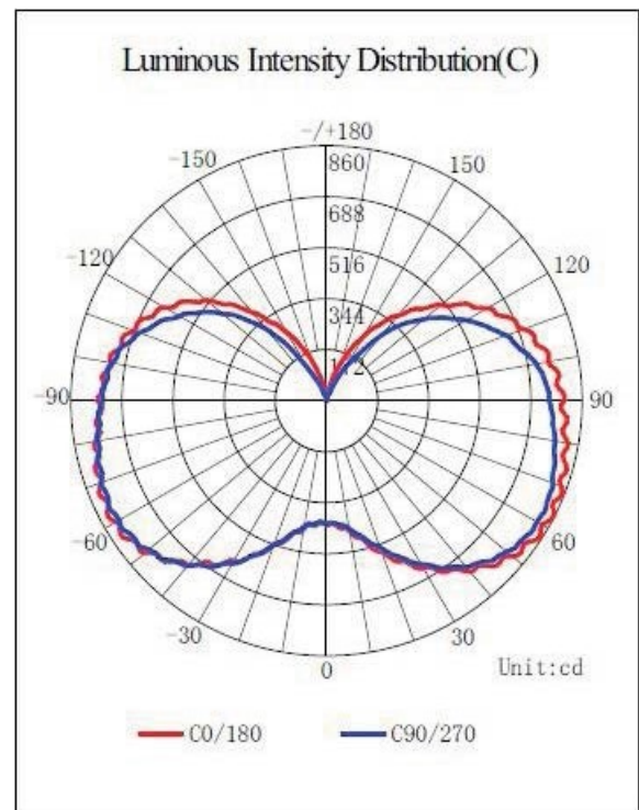
Φ90 Internal Driver 180° Corn Lamp:
