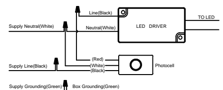
FIG.6.2 Wiring layout with Photocell
