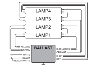
(T5-TYPA wiring diagram)
