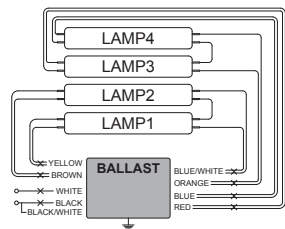
(T5-TYPA wiring diagram)
