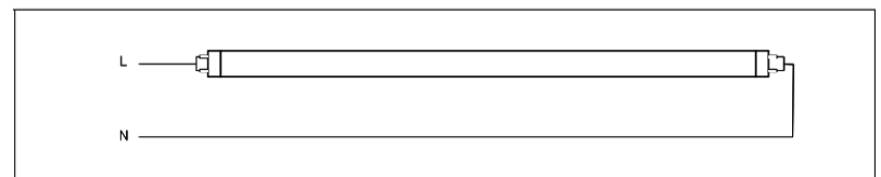
(T8 8ft. wiring diagram)
