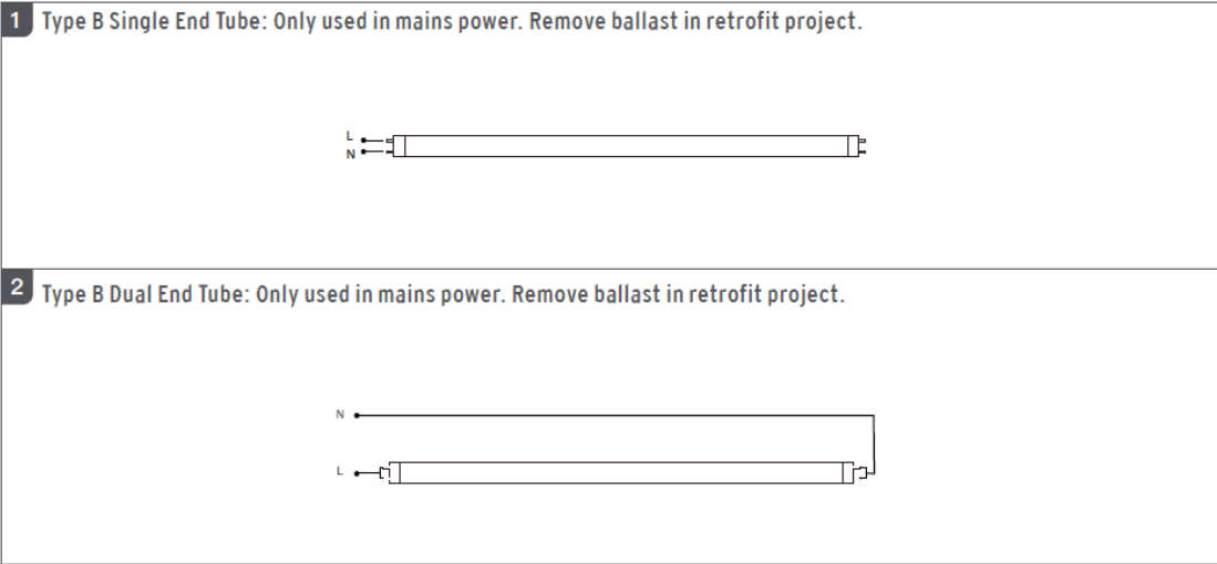
(T8 4ft. wiring diagram)
