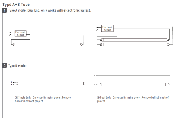
(T8 2ft. wiring diagram)
