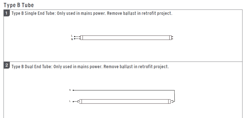
(T8 2ft. wiring diagram)
