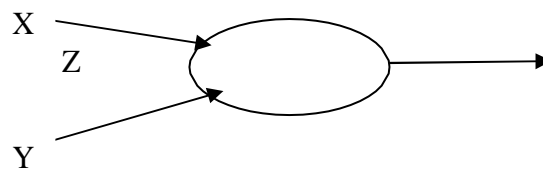
Fig. 4.6 Context Diagram
