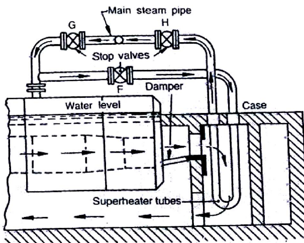
Fig. 3.15 Superheater
