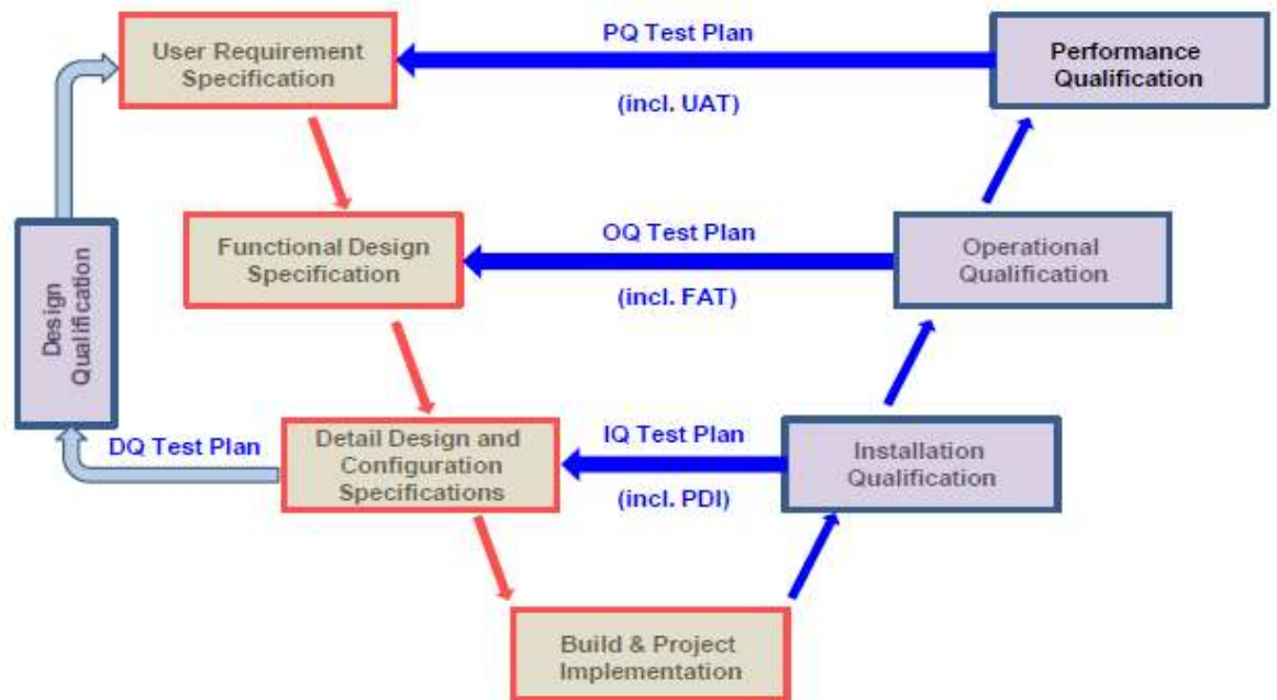
Figure 8 V-model
