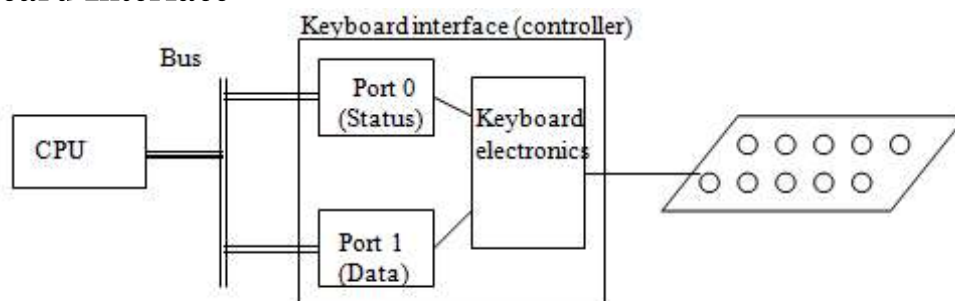
Figure 3. Keyboard controller
