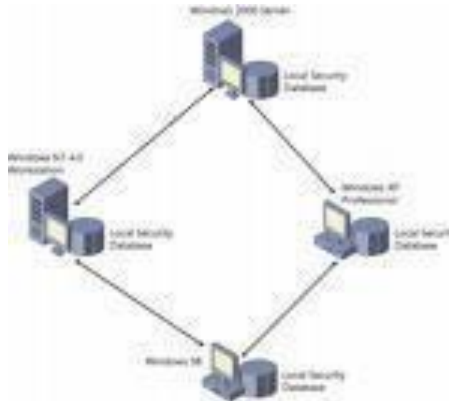
[Peer-Peer architechcer]
