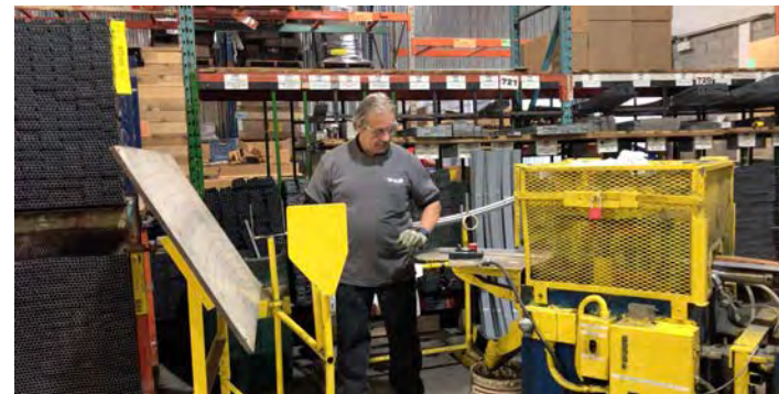
Profilage des composantes de la structure. Profiling of structural components.
