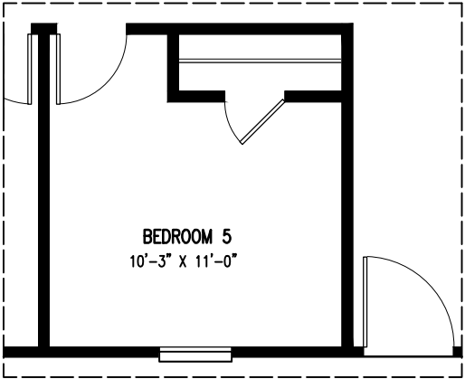
BEDROOM 5 OPTION
