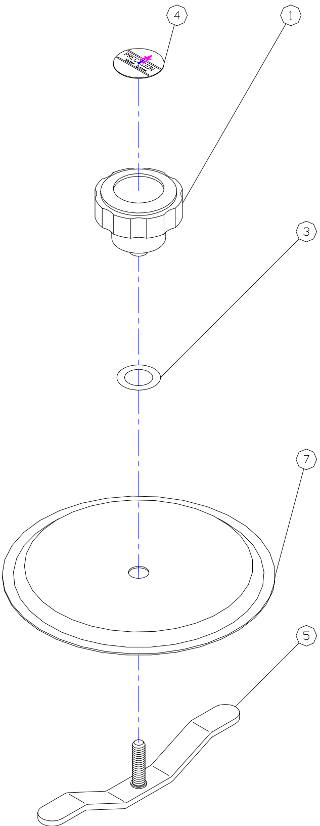
HOLDING TANK LID ASSEMBLY (PART # 500248)
