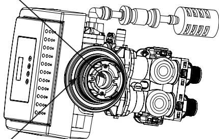
Tank Seal O-ring
