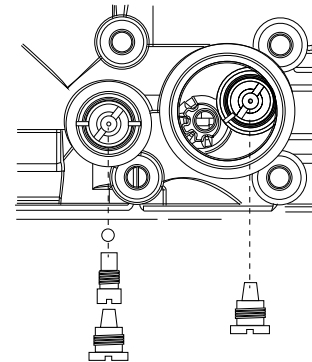
Downflow Injector Configuration
