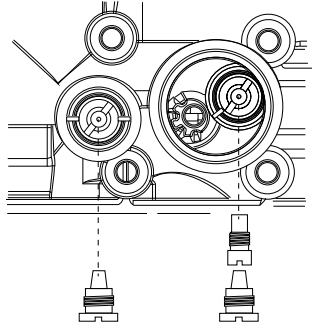
Downflow Injector Configuration
