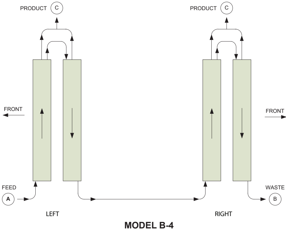
Figure 6. MacRO Module Tubing, two to four membranes.
