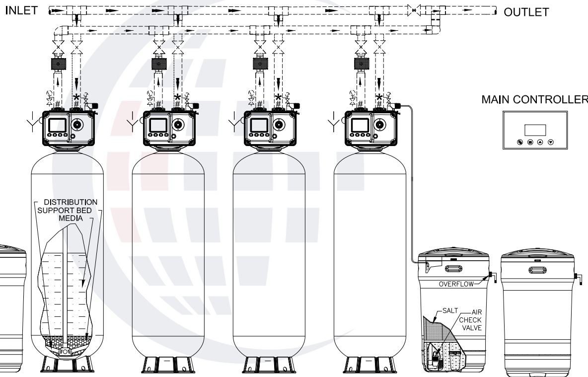
RAW WATER REGENERATION PIPING SHOWN
