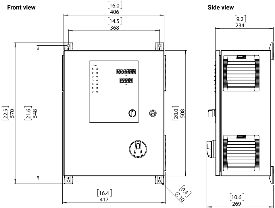
Figure 3: EVEREST Control Panel Dimensions
