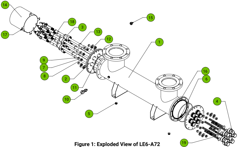
Figure 1: Exploded View of LE6-A72
