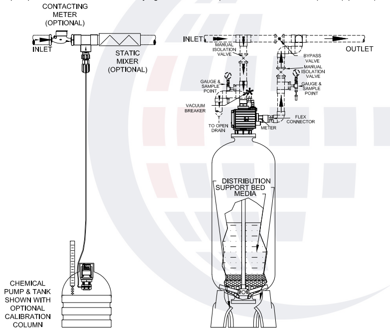
RAW WATER REGENERATION PIPING SHOWN
