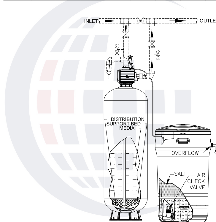
RAW WATER REGENERATION PIPING SHOWN
