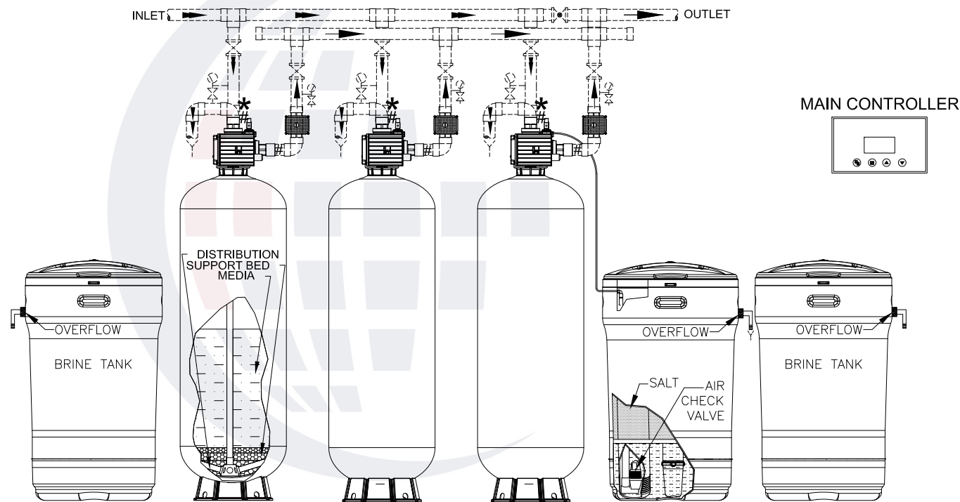
RAW WATER REGENERATION PIPING SHOWN
