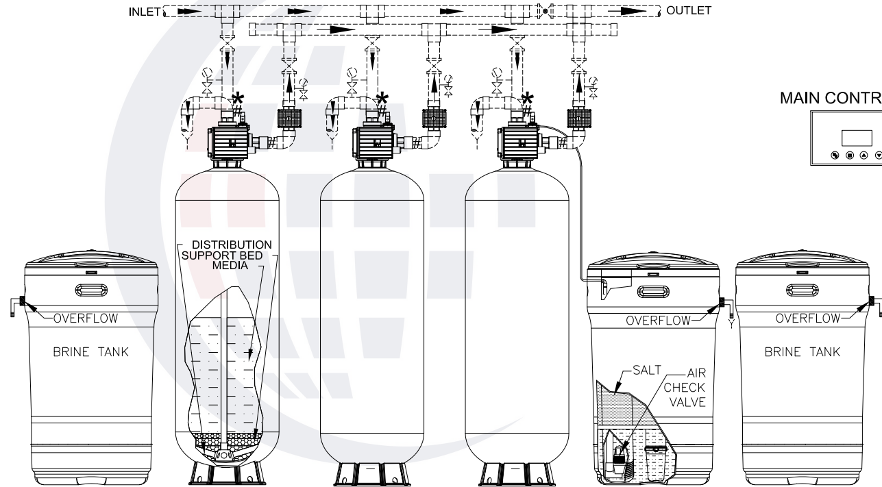
RAW WATER REGENERATION PIPING SHOWN
