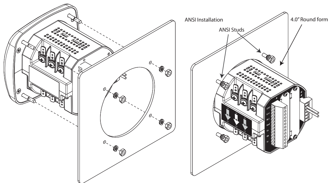
Figure 3.5: ANSI Installation
