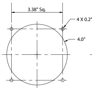
ANSI Mounting
