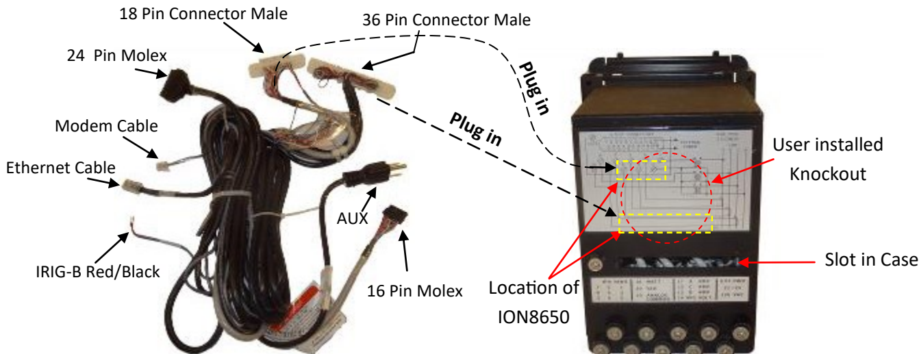
Rear view of Transdata small case
