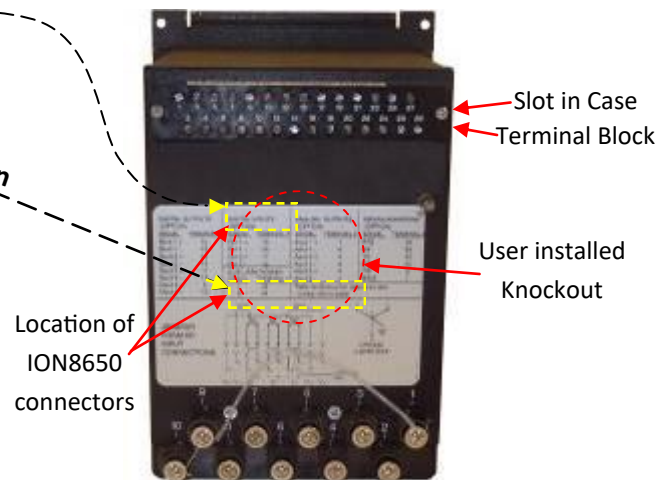
Rear view of JEMSTAR/JEM10 small case
