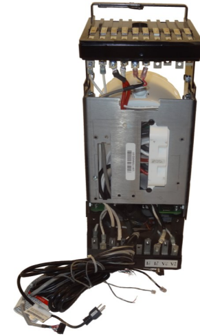
Rear of SWIIGL9-Q1-M8650 with Q1 cable
