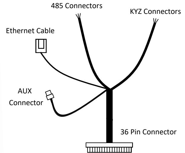
S1K Cable (Custom Cable with AUX, 485, one KYZ, & Ethernet)
