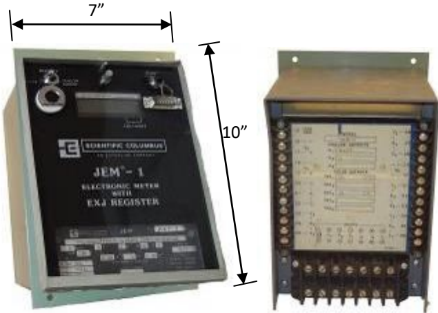
Front and rear view of JEM1 short hardwired case
