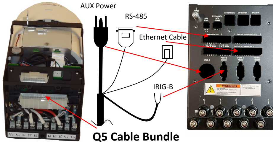
JEMS29 cabling runs through rear of JEMSTAR II case
