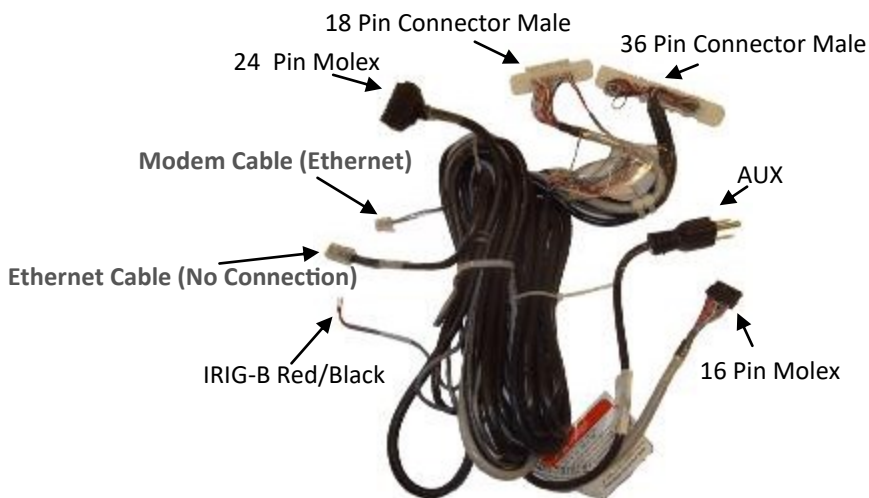
QX1 Cable (Modified FT-21 Cable)
