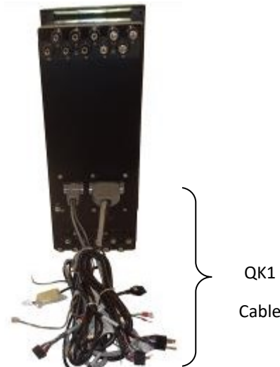
Back of Q1000 Case with QK1 Cables
