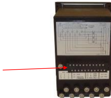
Transdata Module (TM3) connects to back of Transdata case
