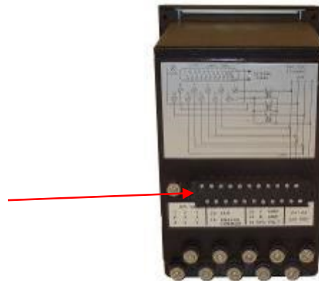
Transdata Module (TM1) connects to back of Transdata case
