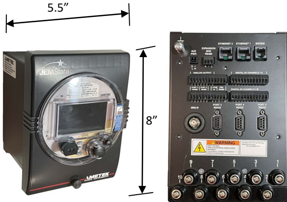
Front and rear view of JEMSTAR II small case
