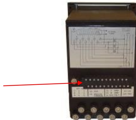
Transdata Module (TM4) connects to back of Transdata case
