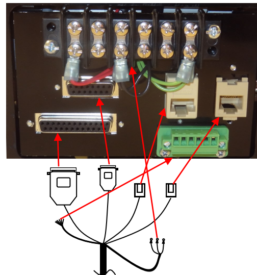
Rear View of QUAD 4 case with installed SWIWM9-Q4A-M8650
