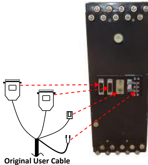
Rear view of JEM2 Tall Case with Original user cables
