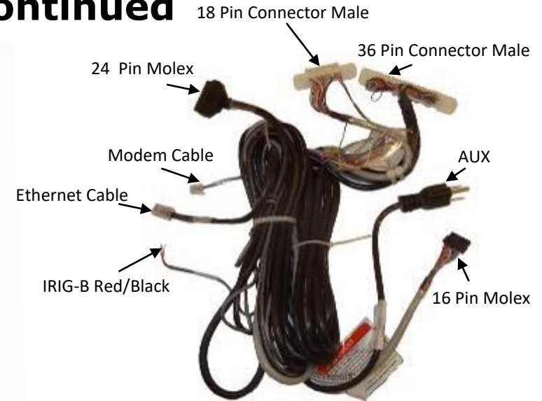
Q1 Cable (Original FT-21 Cable) (Schneider #C0H6C7B & C0H6C7C)
