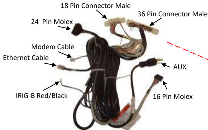
Q1 Cable (Original FT-21 Cable) (Schneider #C0H6C7B & C0H6C7C)
