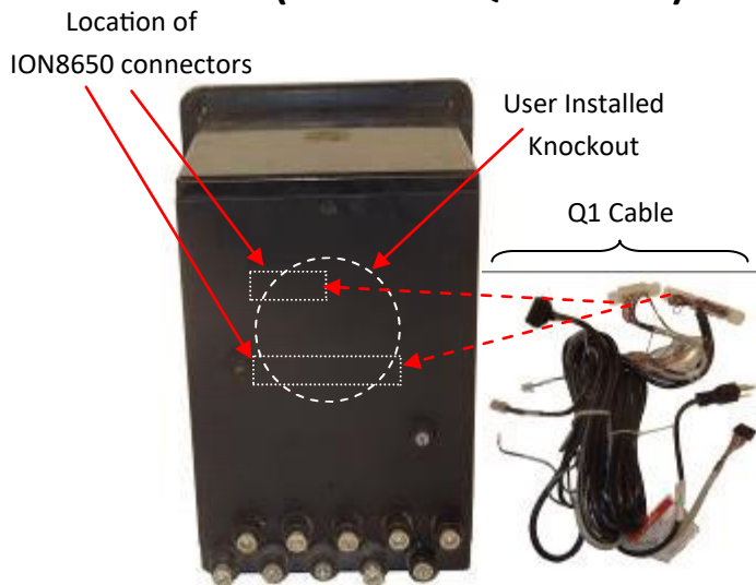
Rear View of DS-65 meter in S1 case with ION 8650 and Q1 Cable
