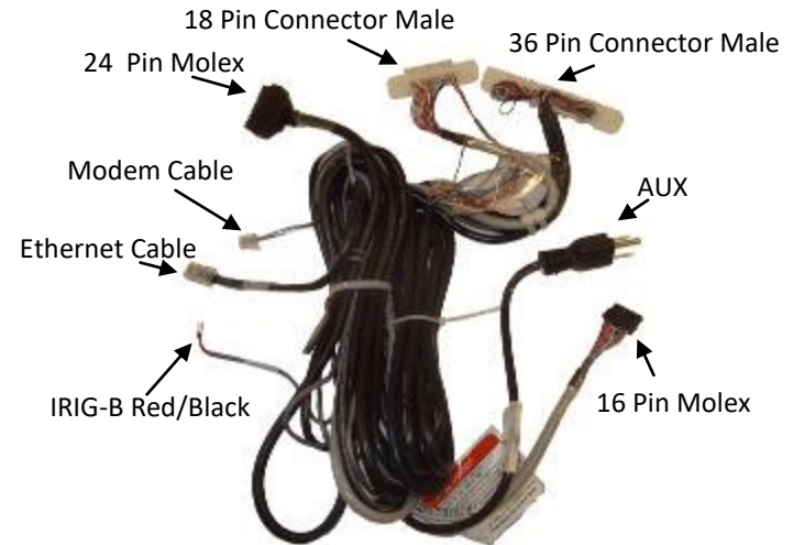
Q1 Cable (Original FT-21 Cable) (Schneider #C0H6C7B & C0H6C7C)
