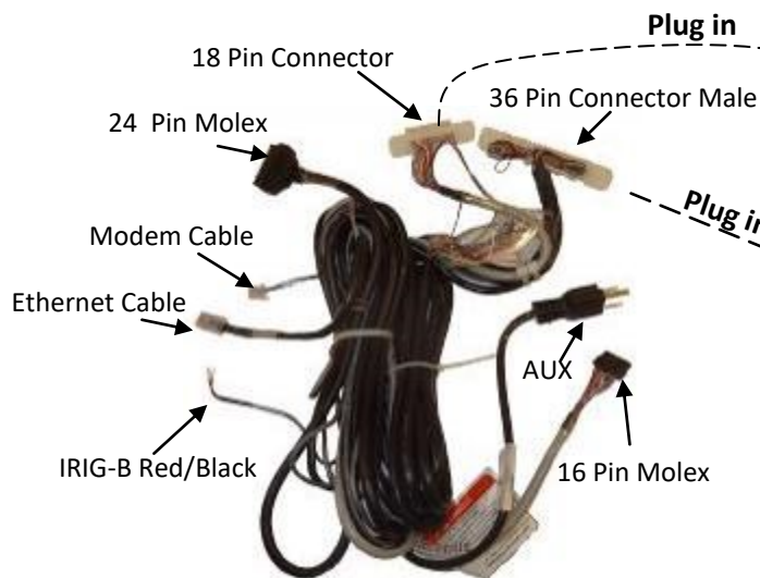
Q1 Cable (Original FT-21 Cable) (Schneider #C0H6C7B & C0H6C7C)
