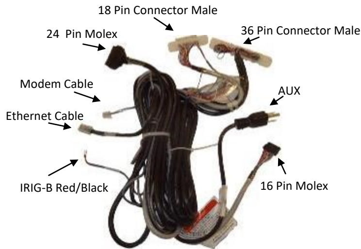
Q1 Cable (Original FT-21 Cable) (Schneider #C0H6C7B & C0H6C7C)
