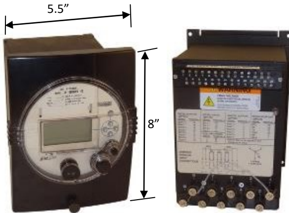
Front and rear view of JEMSTAR/JEM10 small case
