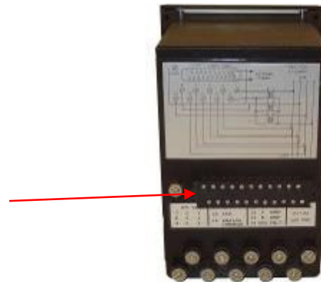
Transdata Module (TM2) connects to back of Transdata case
