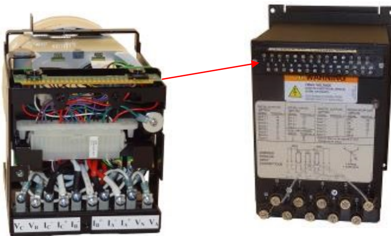
JEMS24 Module connects to back of JEMSTAR case
